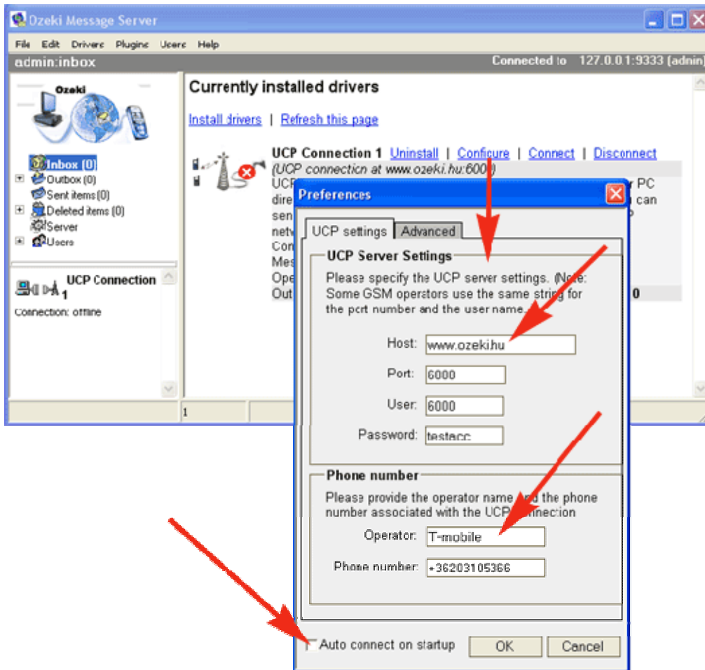
Figure 1. - Configuration of Driver details
