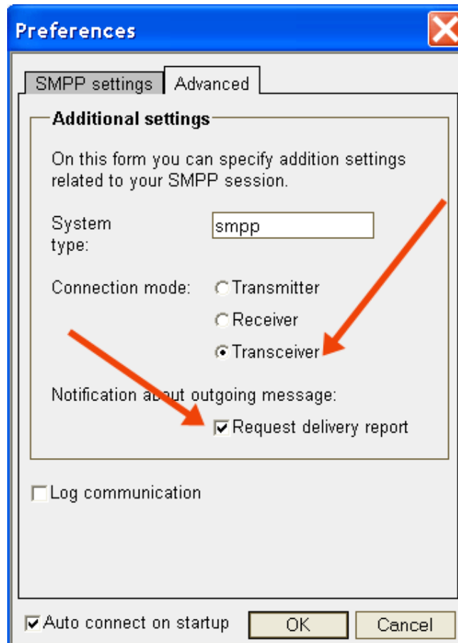
Figure 2. - SMPP advanced
