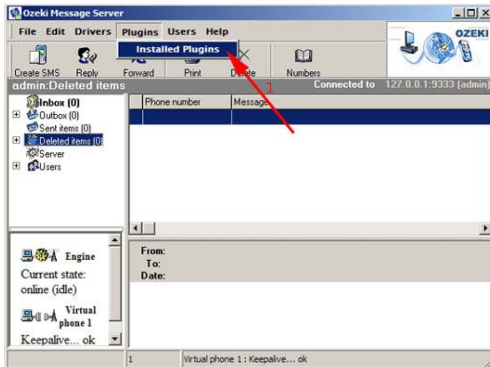
Figure 6 - Installation plugins
