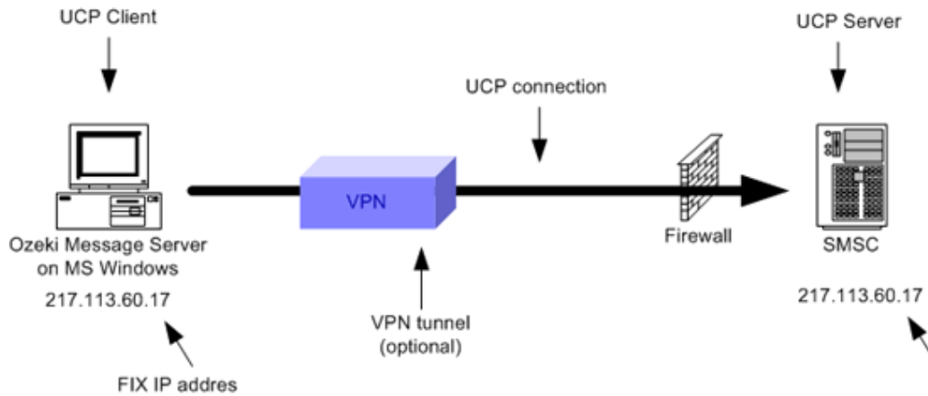
Figure 1 - UCP connection with VPN
