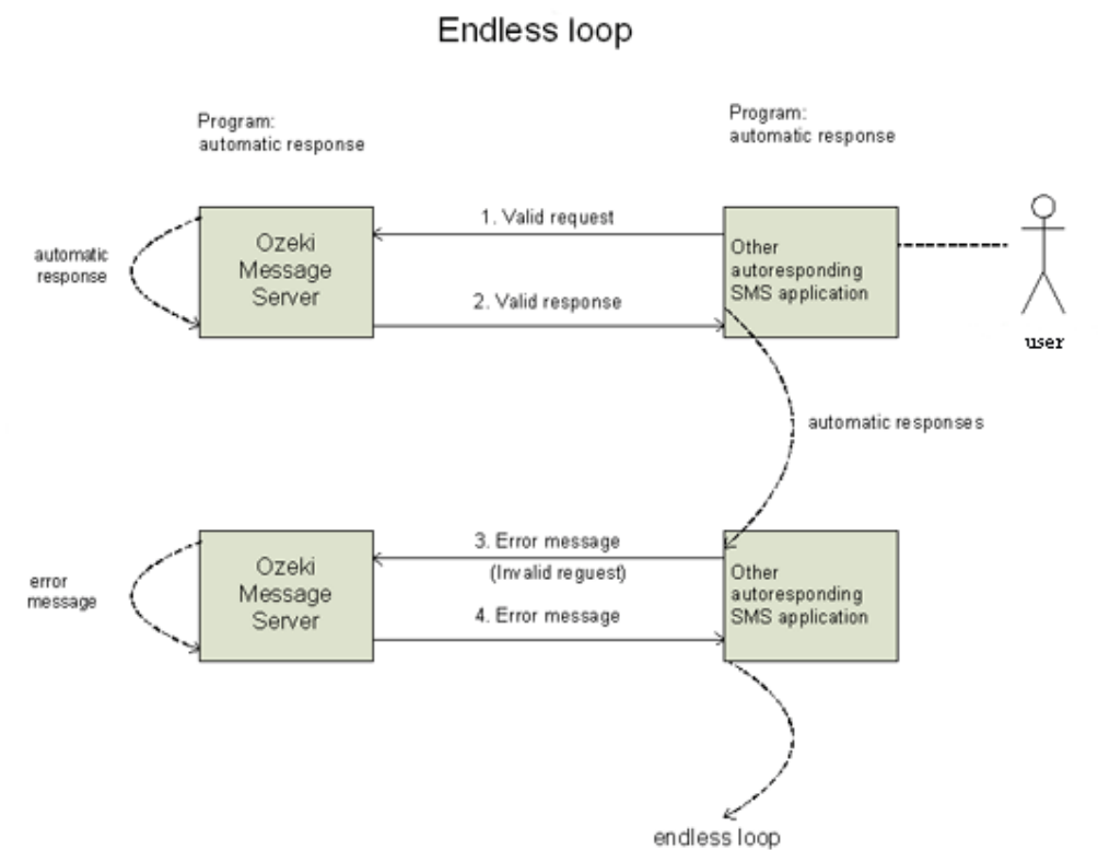
Figure 1 . - Two SMS applications in an endless leep
