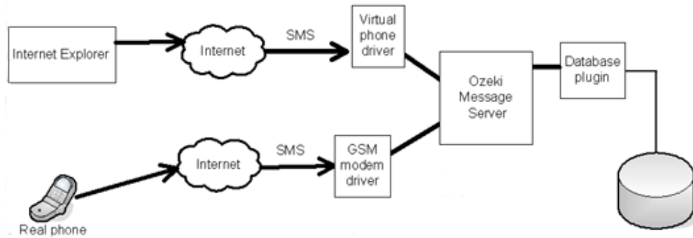
Figure 1. - Virtual phone for developers
