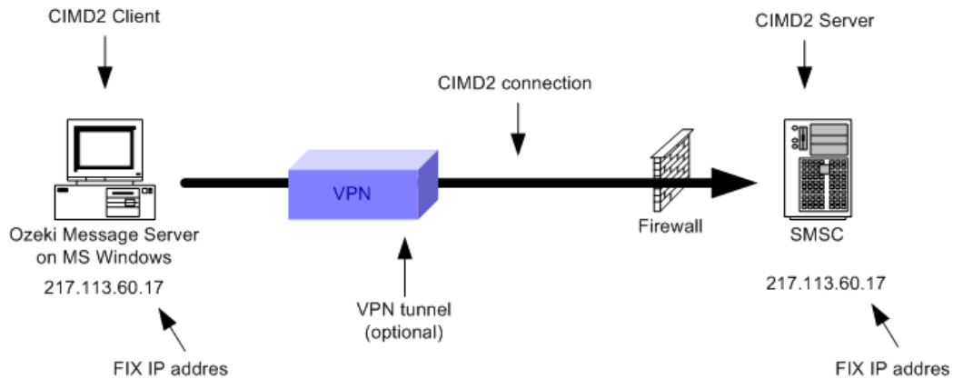
Figure 1 - CIMD2 connection with VPN protection
