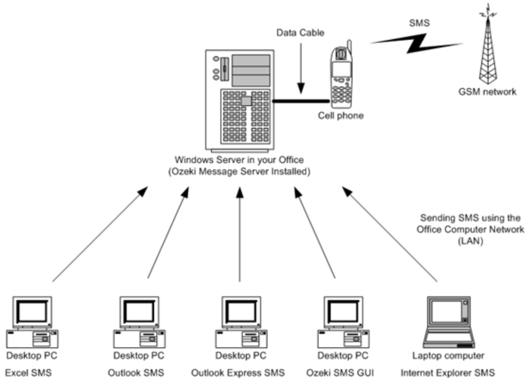
Figure 1 - Ozeki Message Server in the office
